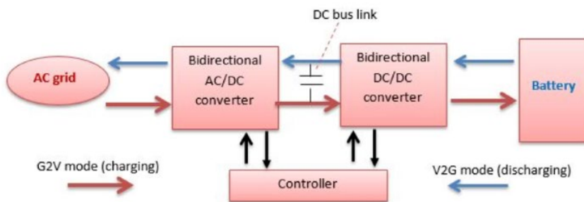
Figure 6: Prototypical bidirectional charger topology.
