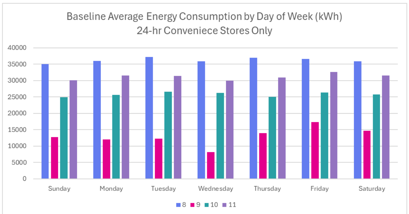
Figure 2: Convenience Store High-Speed Oven Average Energy Consumption
