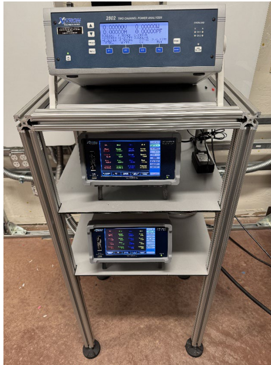
Figure 4: Metering equipment- Xitron 2802 (top) and the two Xitron XT2640AH (bottom)
