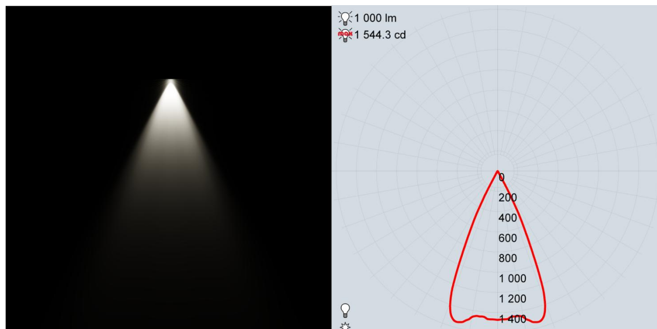
Figure 7: Photometric plot and rendering of fiber emission.
