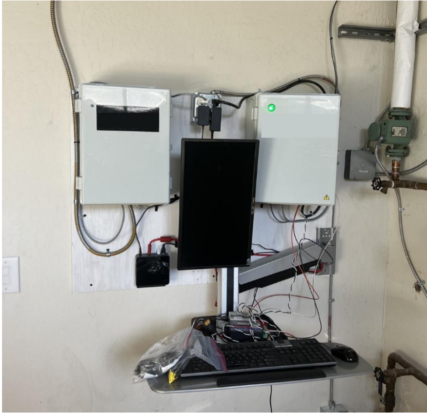
Figure 4: STF control board with power monitoring equipment.
