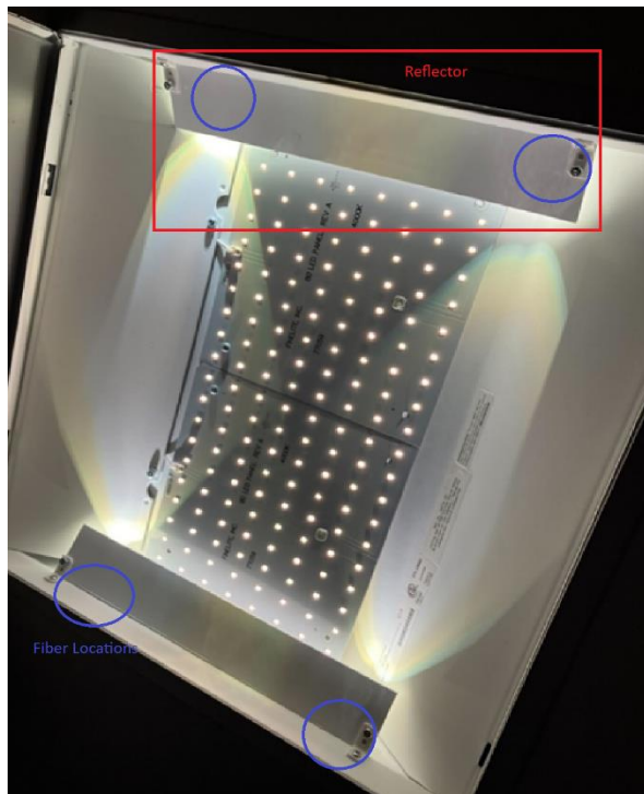
Figure 8: Hybrid fixture without lens.
