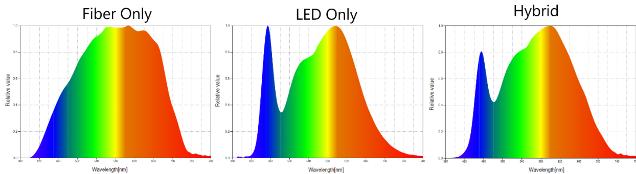
Figure 23: Relative spectral power distribution of the hybrid fixture.
