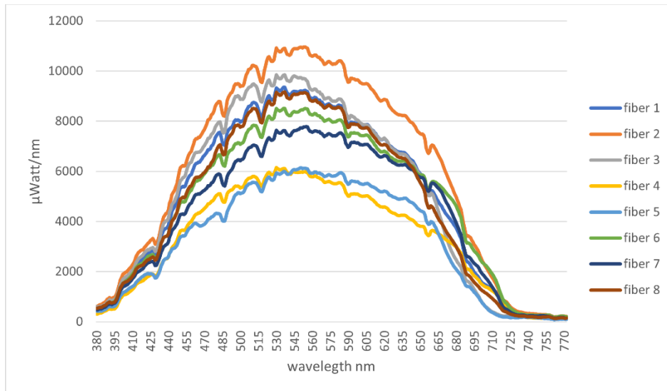
Figure 21: Spectral power distribution of 8 fibers taken within 15 minutes of solar noon on the same sunny day.
