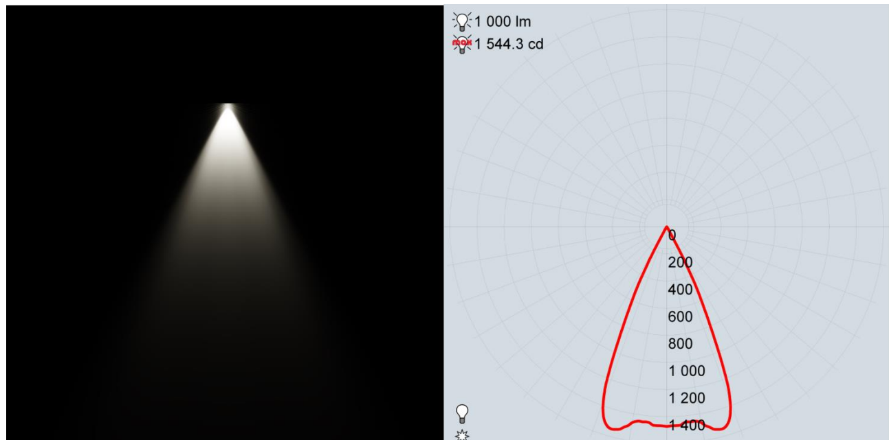
Figure 7: Photometric plot and rendering of fiber emission.
