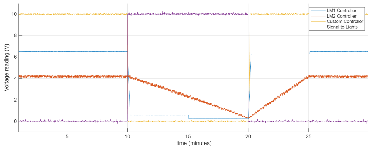
Figure 11: Control system responses to lights being turned on and off in the test space.
