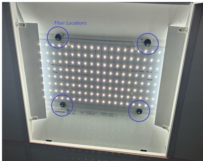
Figure 9: Redesigned fixture with straight-down fiber mounting.
