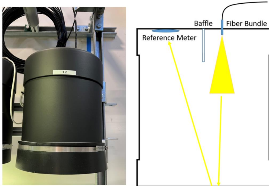
Figure 19: Illuminance test chamber.
