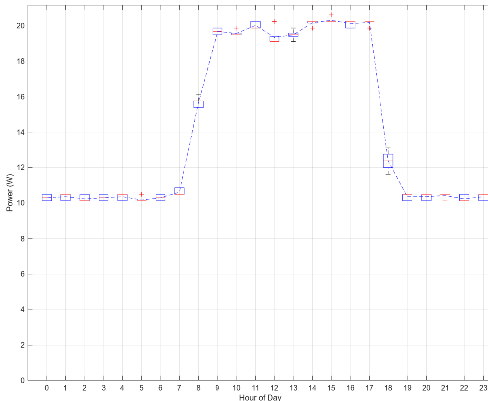
Figure 24: Power draw of STF solar tracker system over the day, with variability at each hour shown.
