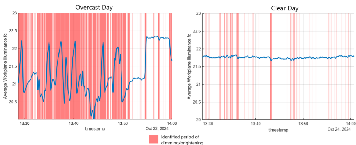
Figure 25: Algorithm output showing dimming and brightening events in work plane illuminance data under overcast conditions.
