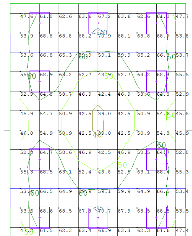
Figure 5: Lighting modeling for the hybrid luminaire system.
