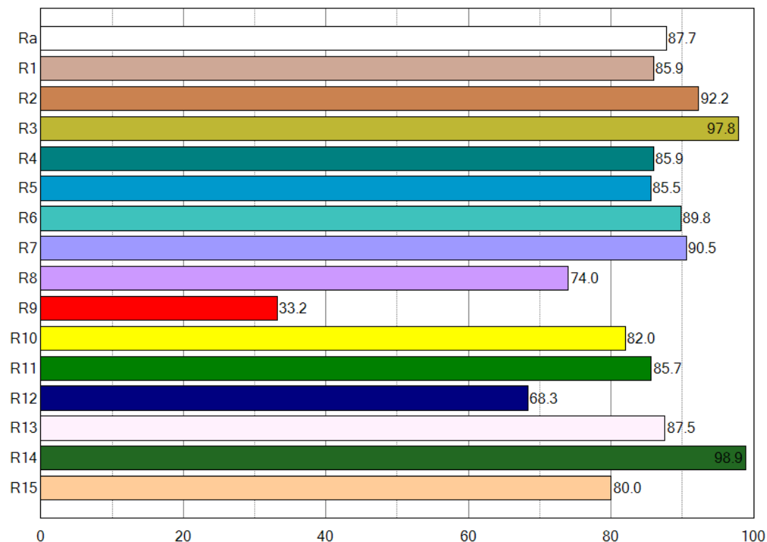
Figure 22: Color rendering results of the hybrid fixture in hybrid configuration at noon on a sunny day (88)
