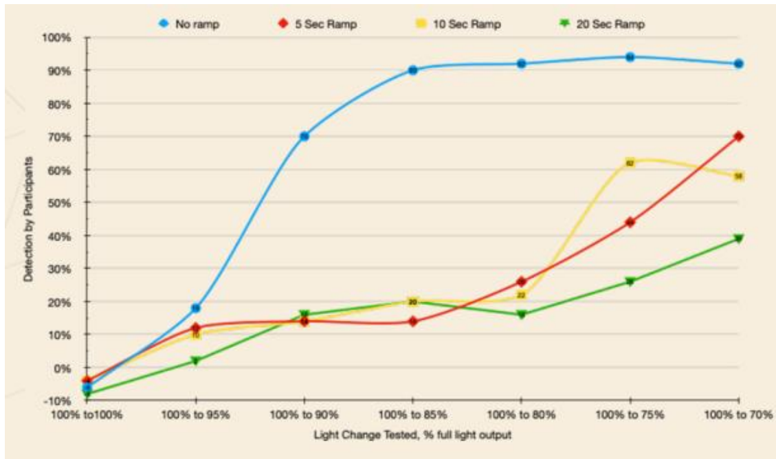
Figure 26: Probability that fluctuations are noticeable in the central vision.
