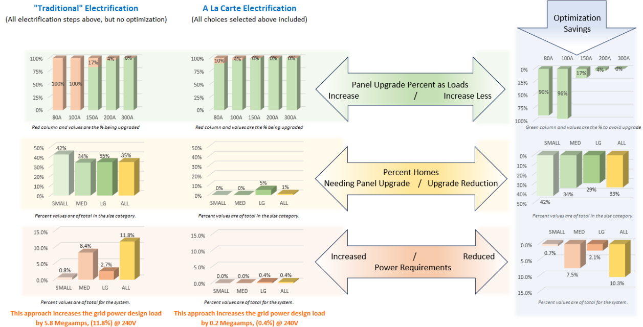
Figure 23. The “Dashboard A La Carte” screen in detail, showing the results.
