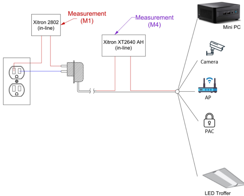
Figure 7: Measurement scheme 3 for the power adapters/bricks for each device.
