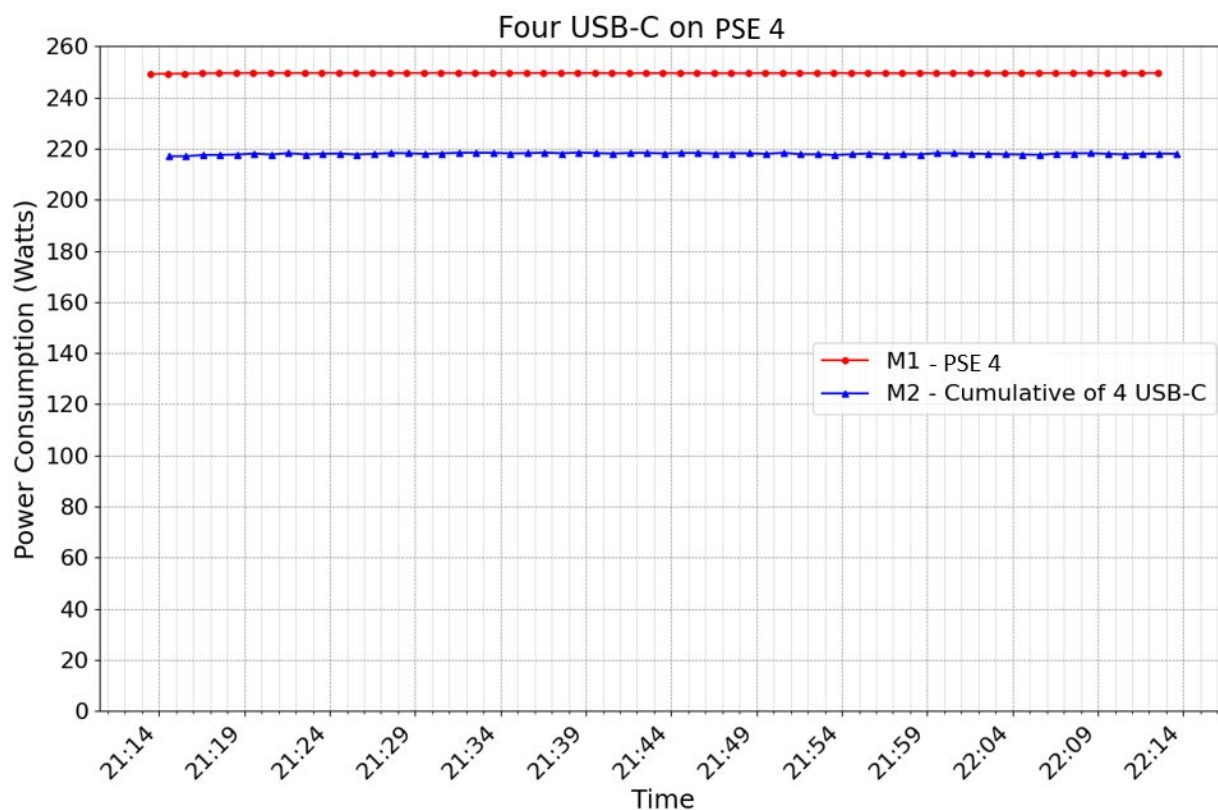
Figure 17. Power consumption of USB-C controller when powered by PoE
