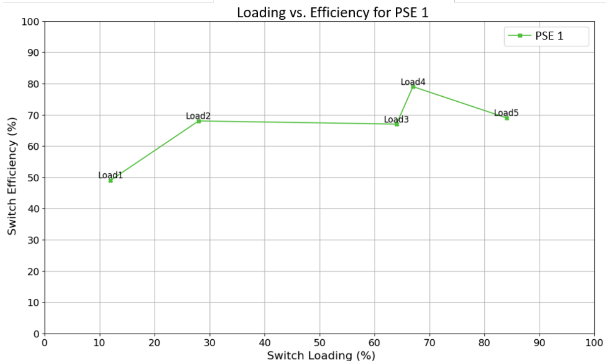
Figure 26: PSE 1 - loading vs. efficiency.
