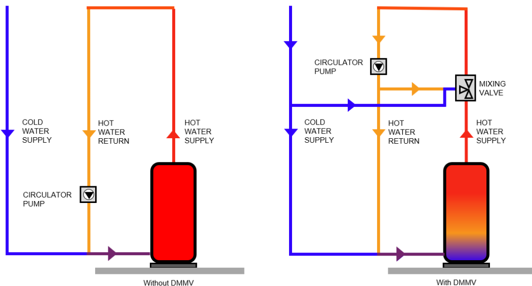
Figure 1: Integrated tank type water heater with and without DMMV.
