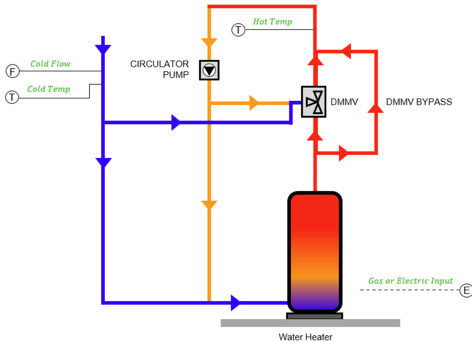
Figure 3: Field-metering Schematic
