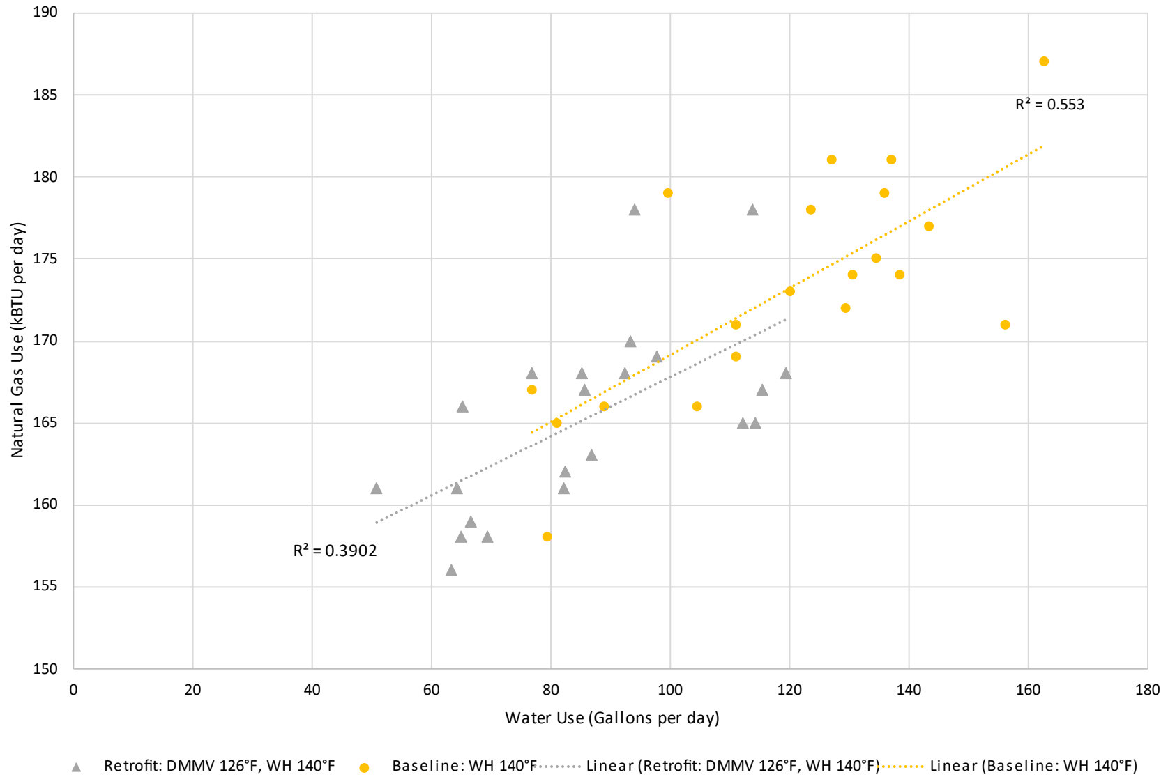
Figure 15: Site 4 Daily Water Use vs. Natural Gas Use
