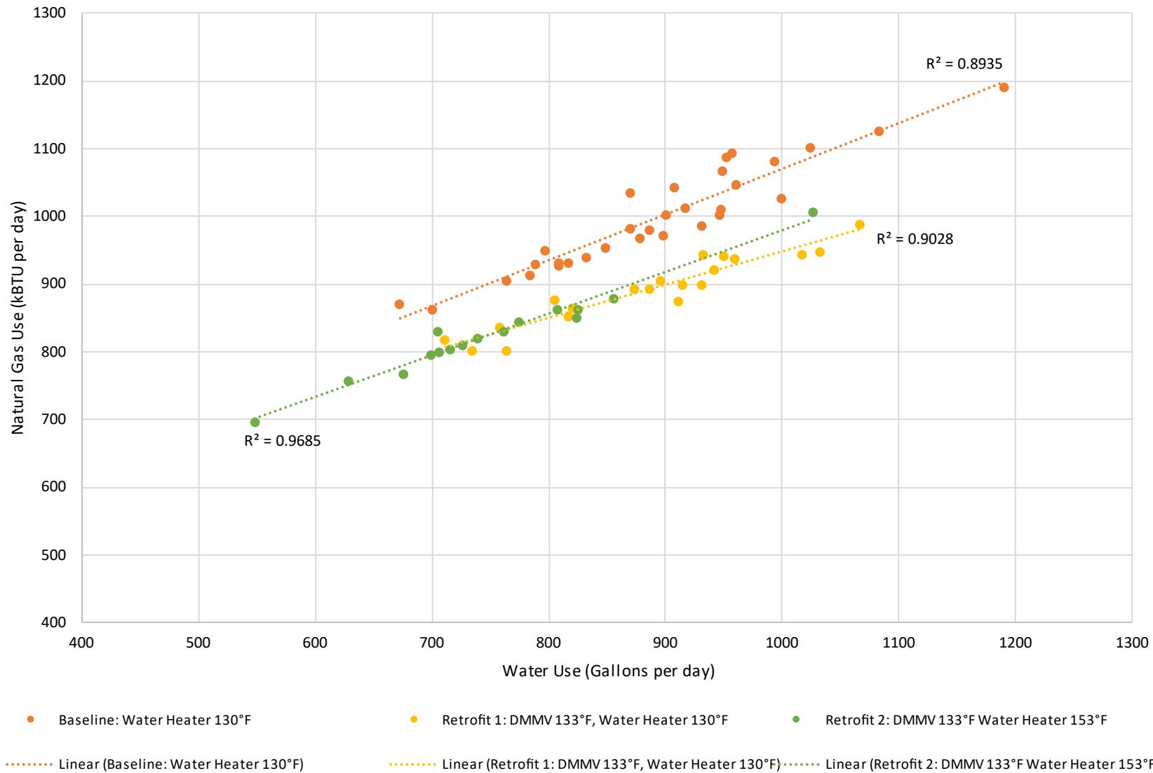
Figure 11: Site 2 Daily Water Use vs. Natural Gas Use
