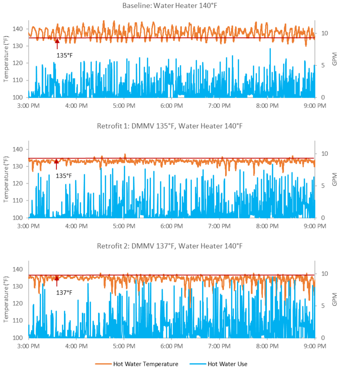
Figure 8: Site 1 DMMV Hot Water Delivery Performance Comparison
