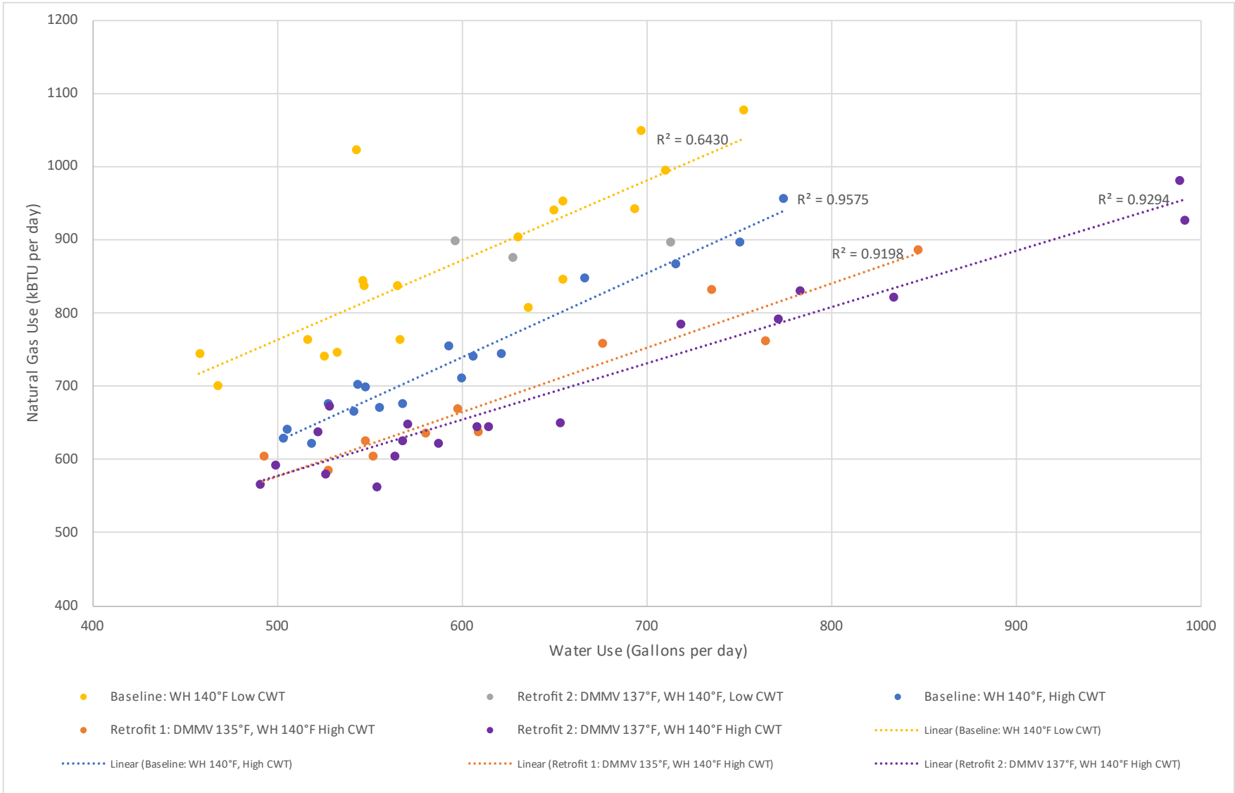
Figure 9: Site 1 Energy Performance
