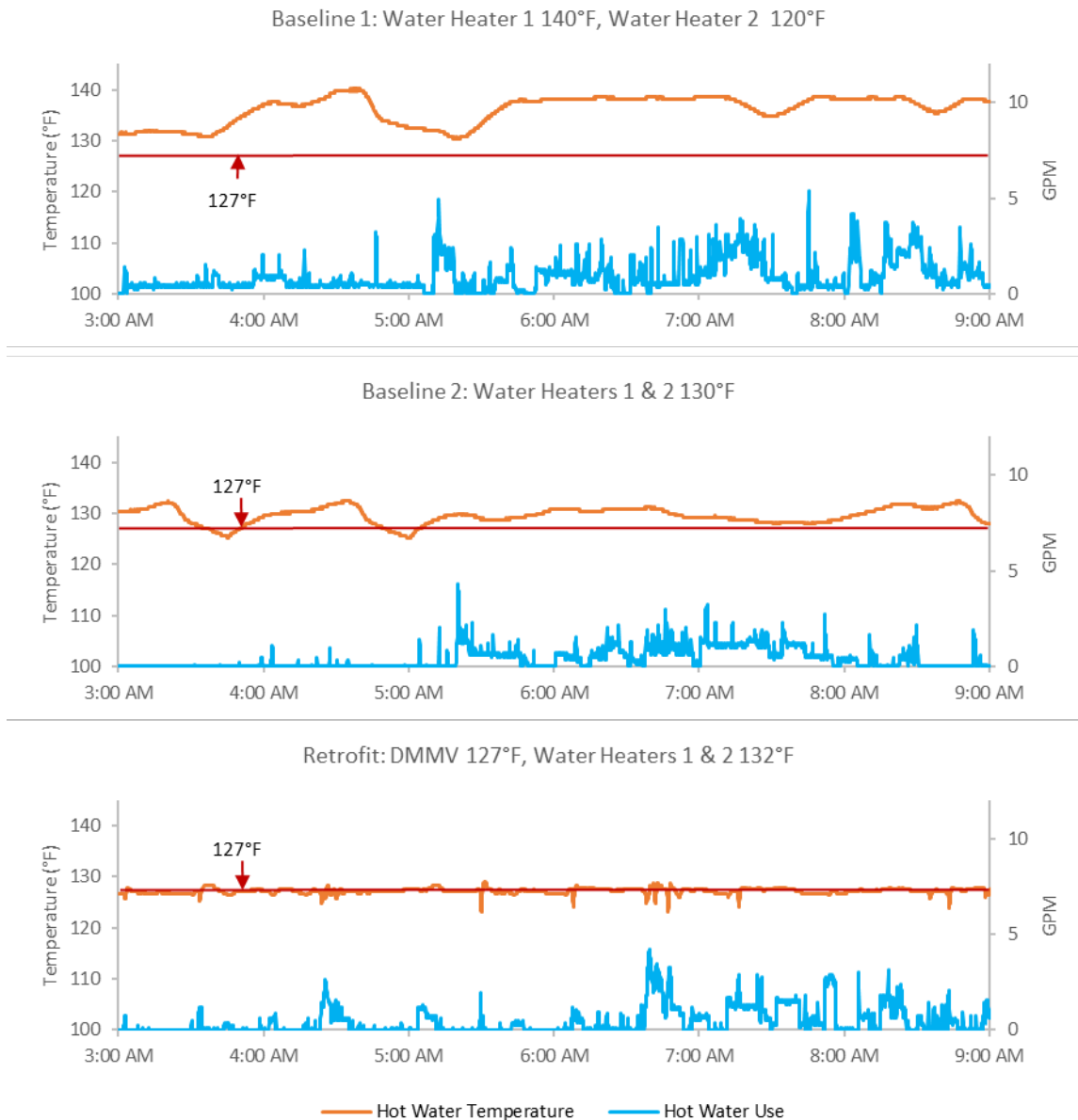
Figure 16: Site 5 Hot water delivery performance
