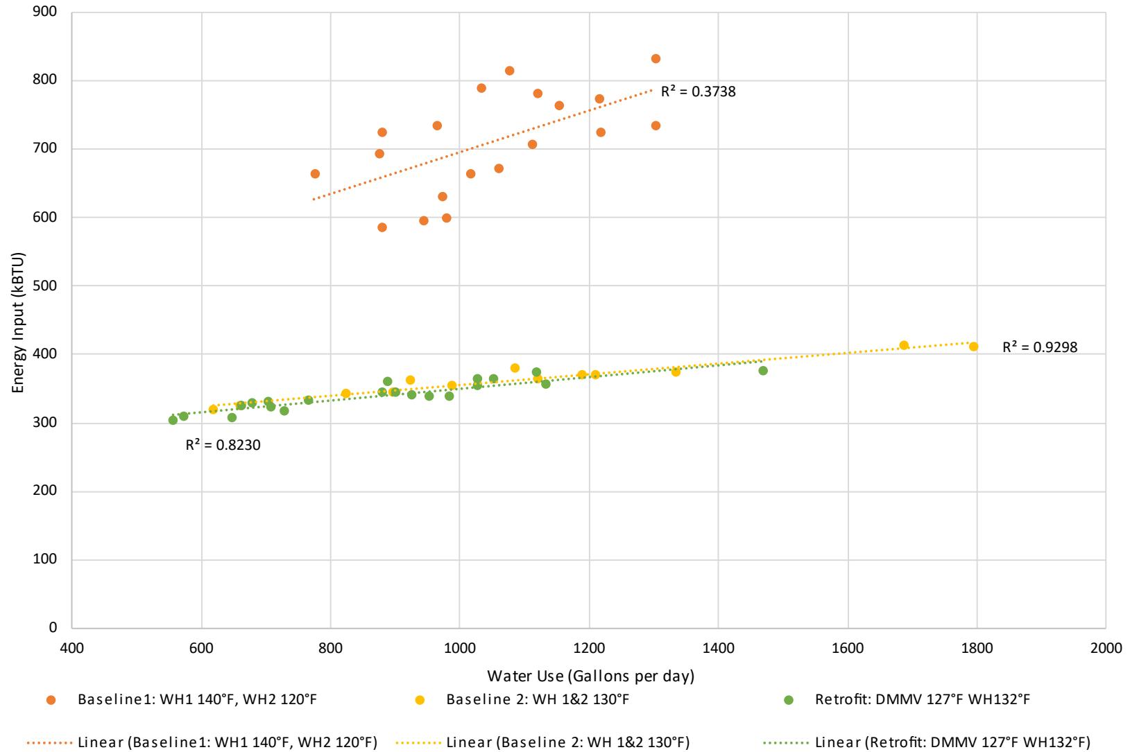
Figure 17: Site 5 Daily Water Use vs. Energy Input
