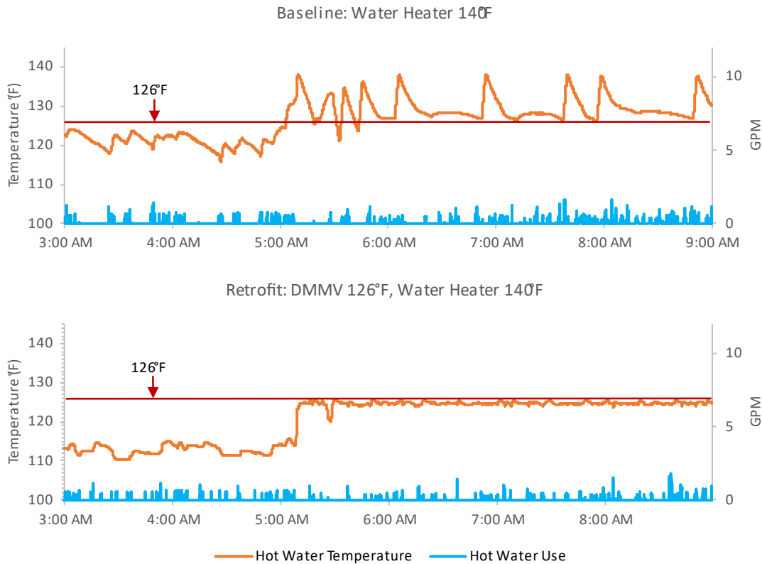
Figure 14: Site 4 DMMV Hot Water Delivery Performance
