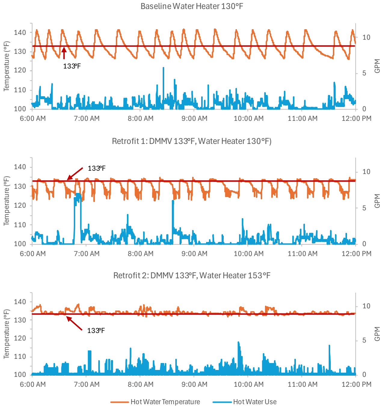
Figure 10: Site 2 DMMV Hot Water Delivery Performance
