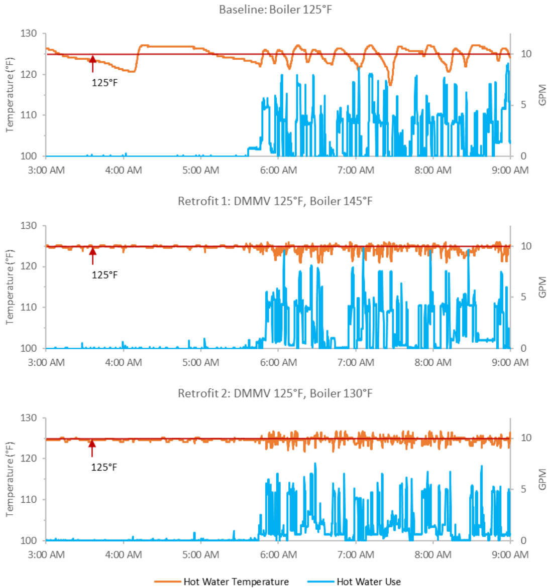
Figure 12: Site 3 Hot Water Delivery Performance
