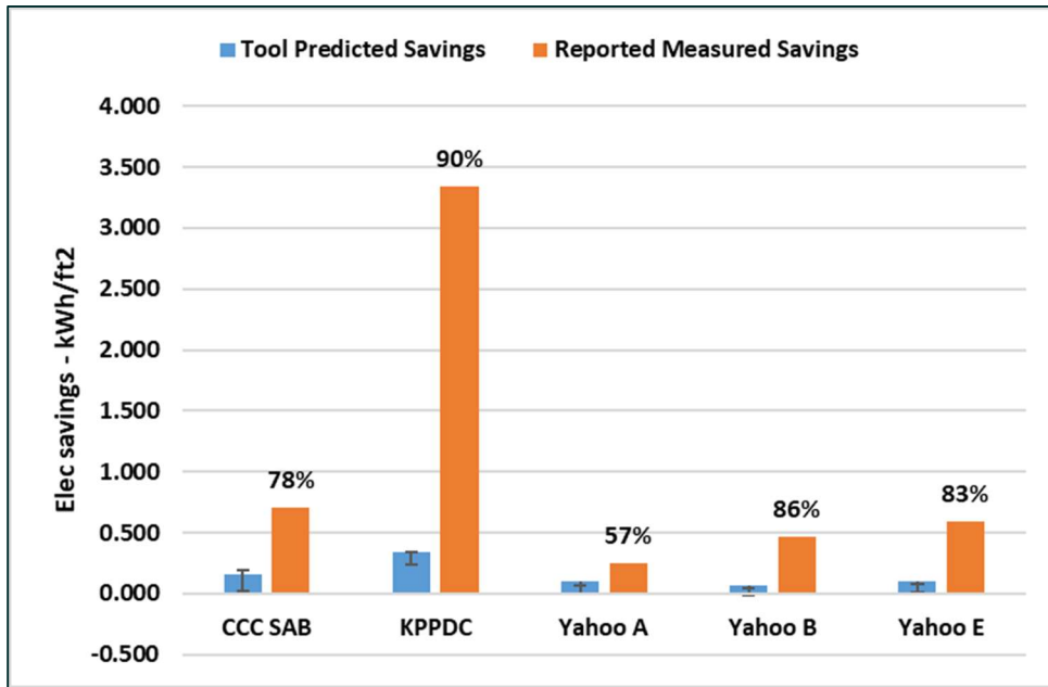
Figure 26: Comparison of Tool Predicted Electricity Savings and Reported Measured Savings for Five Example Sites from EPIC-BiC Project and ASHRAE RP-1515 Project
