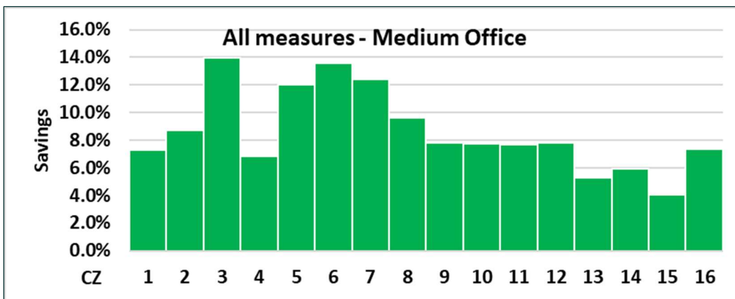
Figure 16: Whole Building Energy Savings Percentage of G36 Measures
